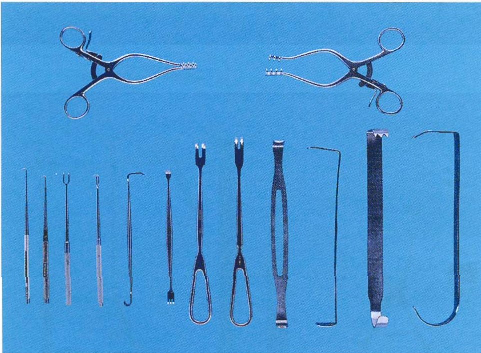
85-4 Top , 2 Weitlaner retractors, sharp prong, medium. Bottom, left to right , 2 Joseph skin hooks, single prong, side view; 2 Joseph skin hooks, double prong, front view and side view; 2 Miller-Senn retractors, side view and front view; 2 Volkmann retractors, 2 prong, sharp; 2 Army-Navy retractors, front view and side view; 2 Hibbs laminectomy retractors, narrow, front view and side view.
